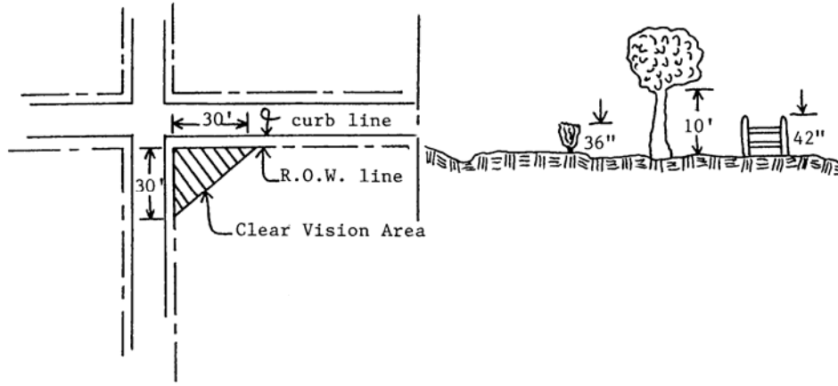
Figure 1 Sight Intersection Triangle
